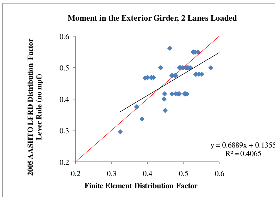
Figure 31. AASHTO LRFD, Moment - Exterior Girder 2 Lanes Loaded
