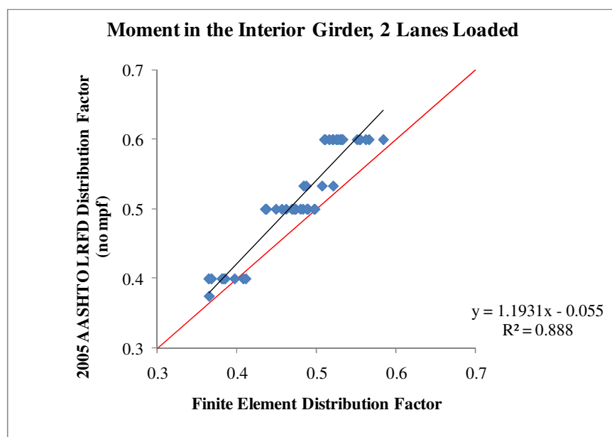
Figure 17. AASHTO LRFD, Moment - Interior Girder 2 Lanes Loaded
