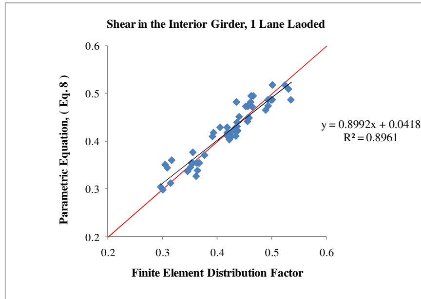
Figure 26. Proposed Equation, Shear - Interior Girder 1 Lane Loaded
