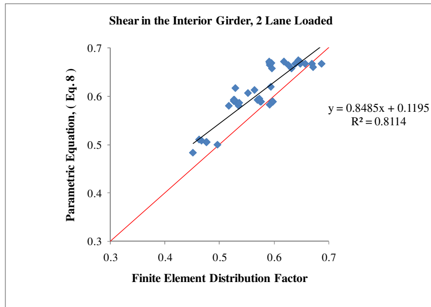
Figure 27. Proposed Equation, Shear - Interior Girder 2 Lanes Loaded
